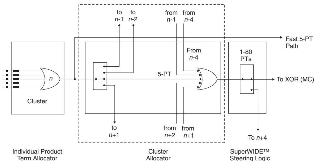
Figure 4. Macrocell Slice
