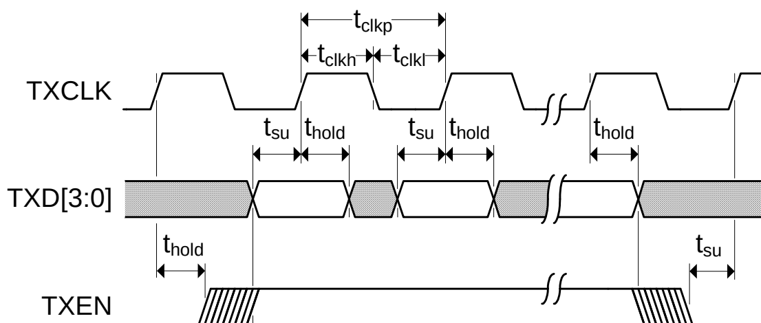
Figure 5.5 MII Transmit Timing
