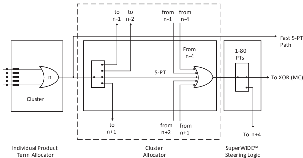
Figure 4.3. Macrocell Slice
