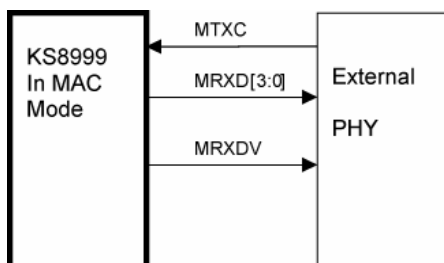
Figure 6. Data Sent from KS8999 PHY Mode to External PHY Device
