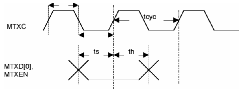
Figure 9. SNI (7-wire) Input Timing
