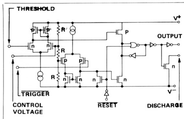
Figure 5. Equivalent circuit.
