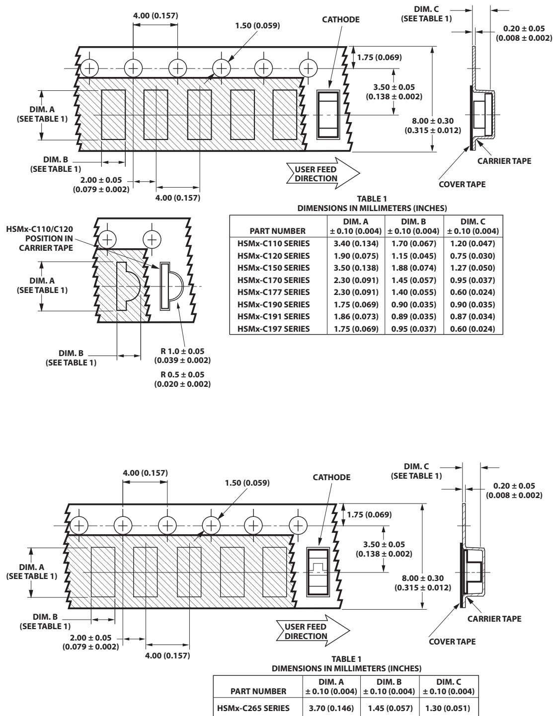
Figure 19. Tape dimensions.
