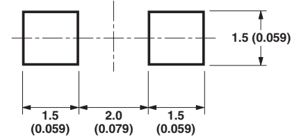
Figure 12. Recommended soldering pattern for HSMx-C150.
