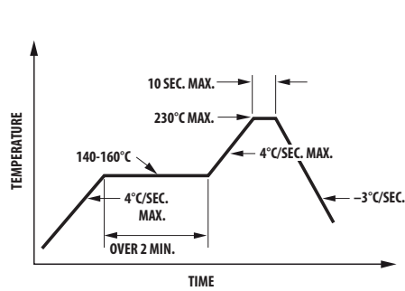
Figure 7. Recommended reflow soldering profile.
