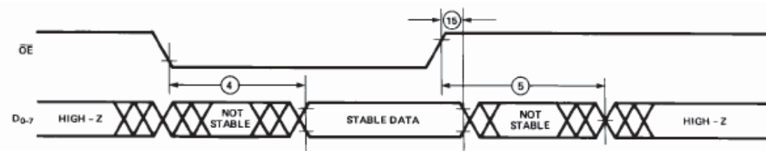
Figure 3: Tri-State Output Timing
