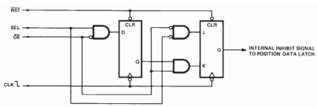
Figure 11. Simplified Inhibit Logic
