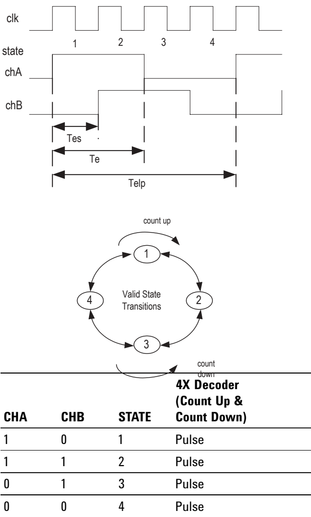
Figure 9. 4x Decoder Mode
