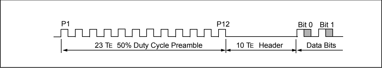
FIGURE 9-5: CODE WORD FORMAT: DATA PORTION
