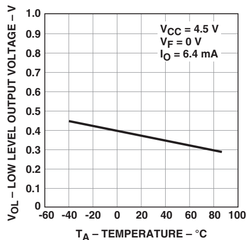
Figure 1: Typical Logic Low Output Voltage Vs. Temperature
