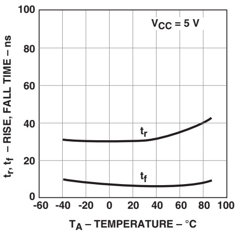
Figure 9: Typical Rise, Fall Time vs. Temperature
