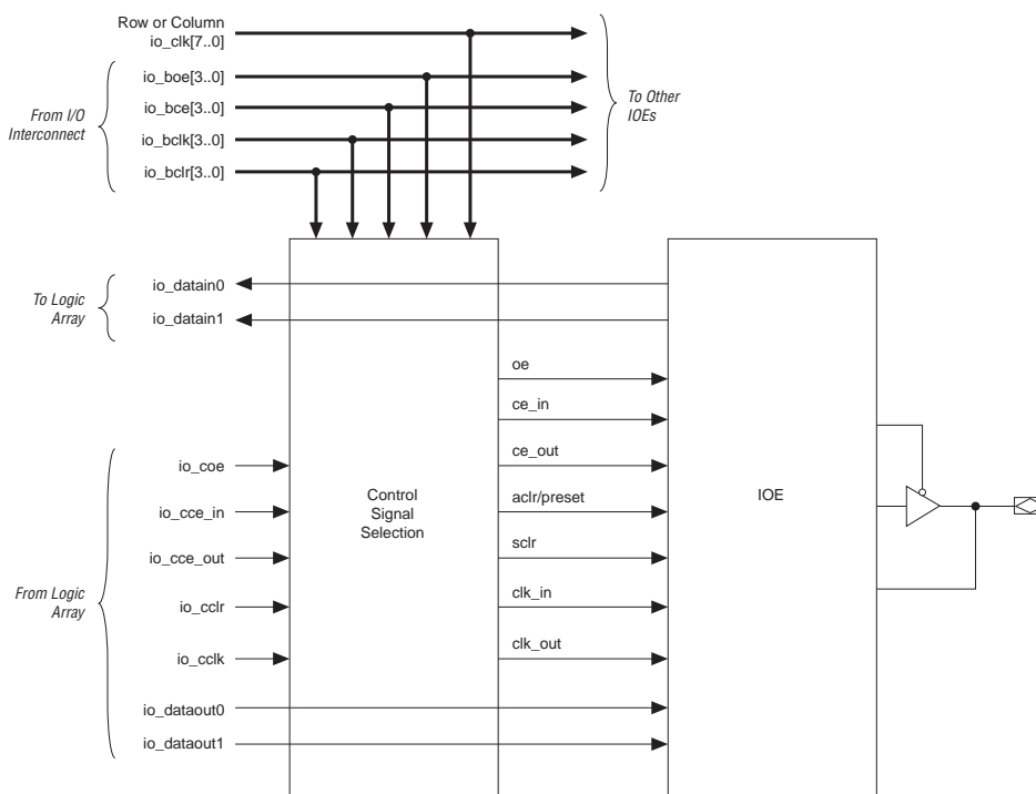
Figure 4-61. Signal Path Through the I/O Block
