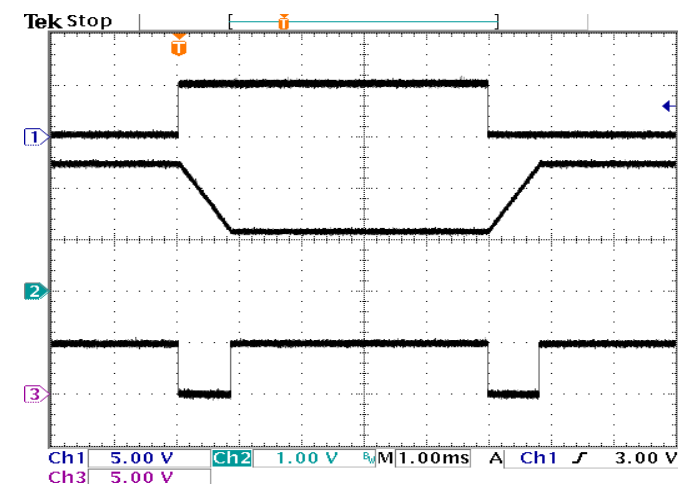
V OUT Scaling with VID Codes at V IN = 5V
