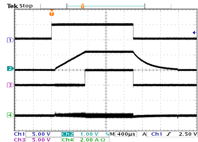
Power Up/Down at No Load: V IN = 5V, V OUT = 1.2V
