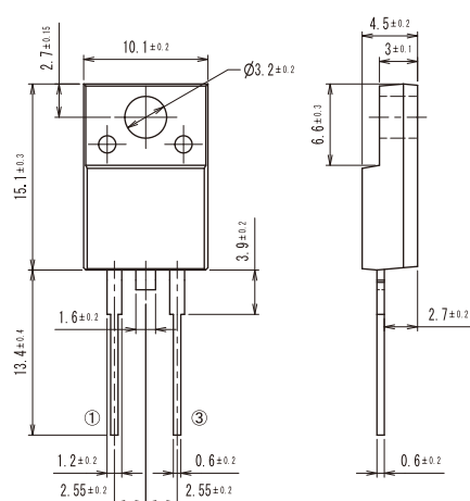
<A-17> TO-220 Full-Mold 2pin
