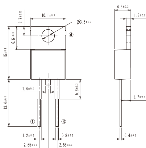
<A-15> TO-220
