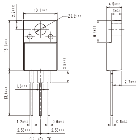
<A-18> TO-220 Full-Mold
