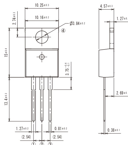
<A-18> TO-220 Full-Mold
