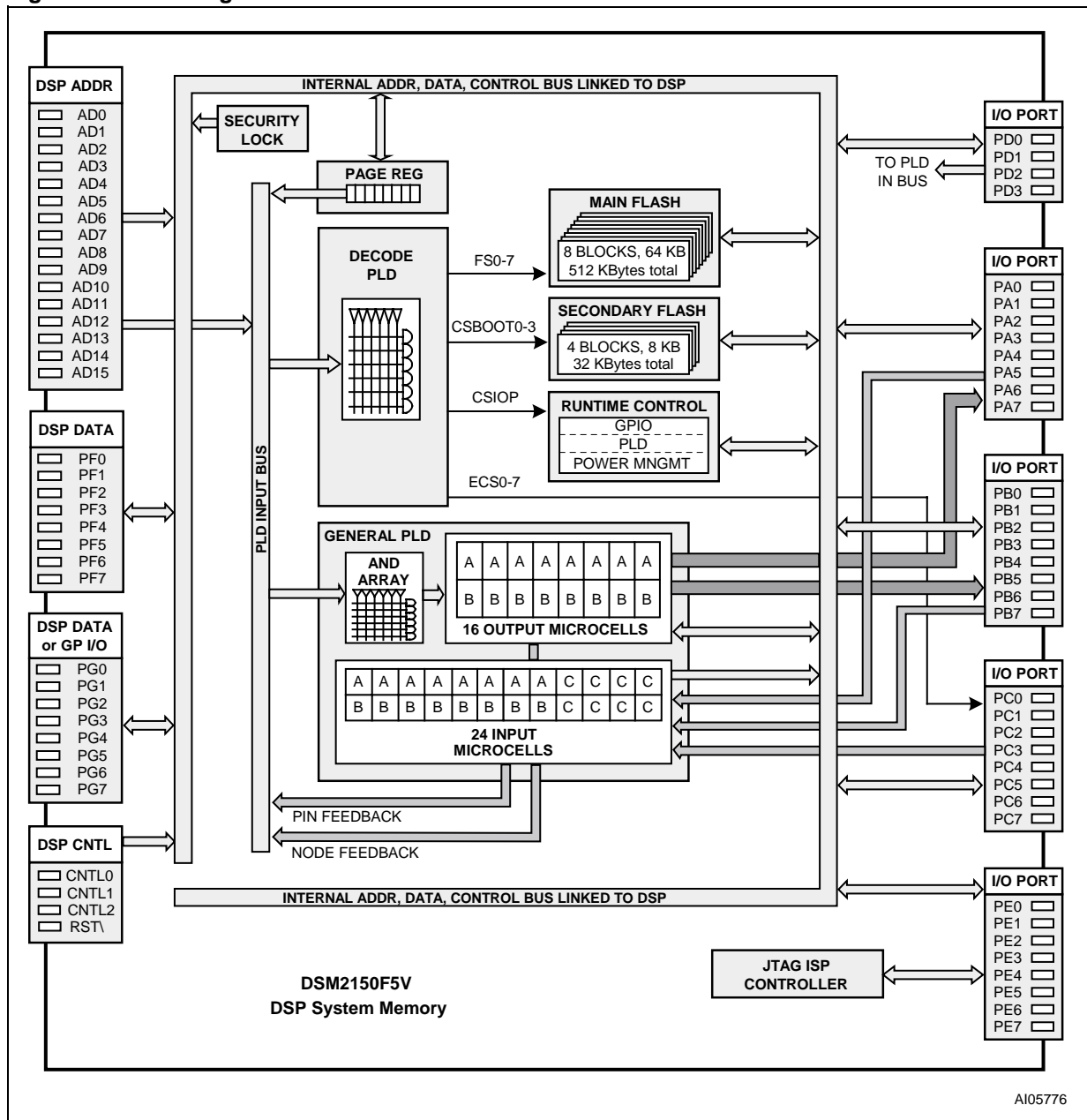
Figure 4. Block Diagram
