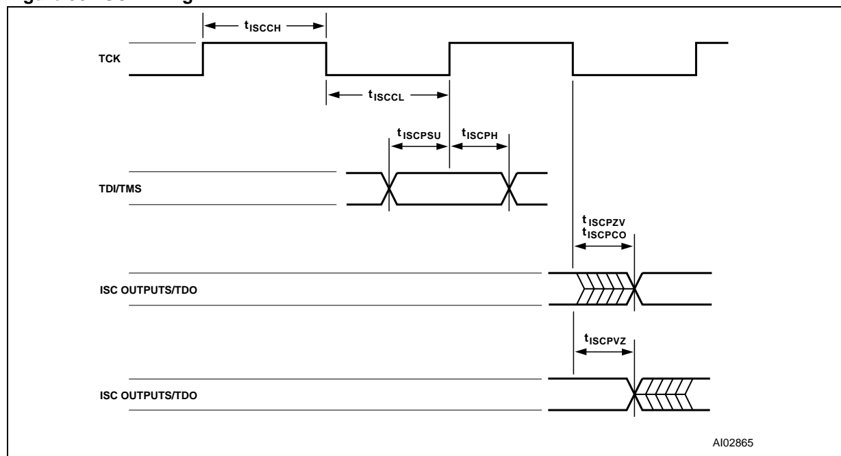
Figure 35. ISC Timing
