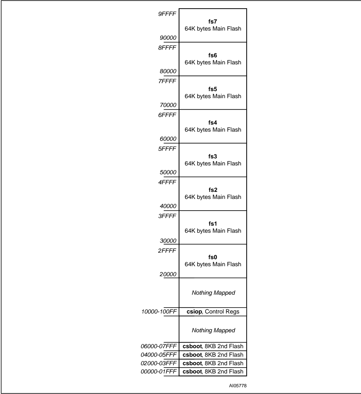
Figure 11. Memory Map, ADSP-21535
