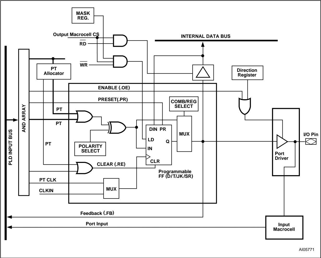
Figure 9. CPLD Output Macrocell
