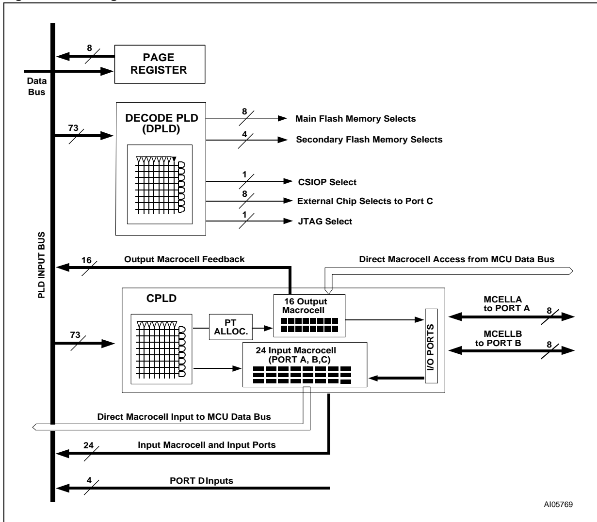
Figure 6. PLD Diagram
