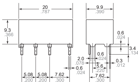
External dimensions
