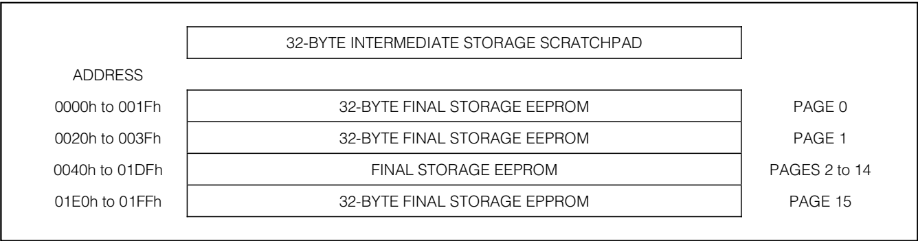
Figure 5. Memory Map
