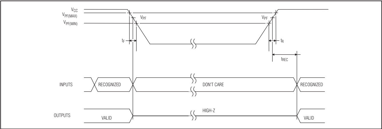
Figure 2. Power-Up/Power-Down Timing
