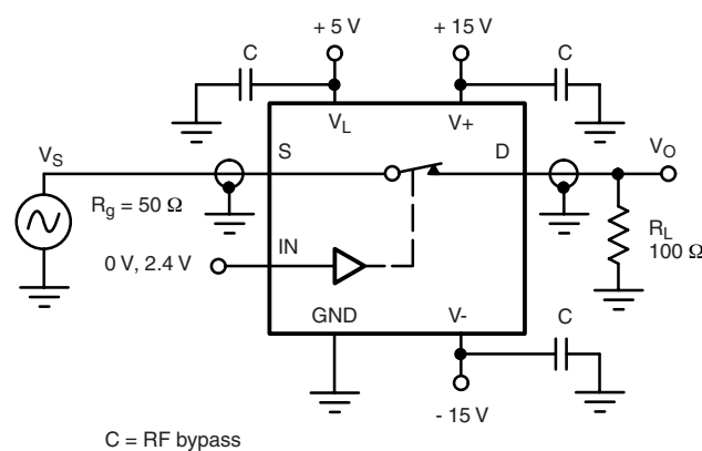
Figure 6. Insertion Loss
