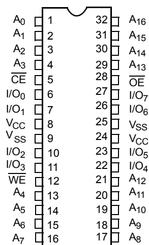
Figure 1. 32-pin SOJ Top View
