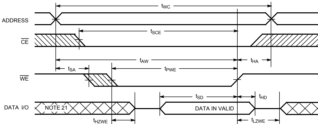
Figure 8. Write Cycle No. 3 ( \overline{\text{WE}} Controlled, \overline{\text{OE}} LOW) [20, 22]
