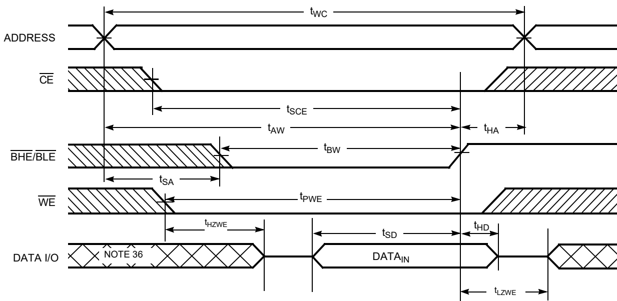
Figure 11. Write Cycle No. 4 ( \overline{\text{BHE/BLER}} Controlled) [33, 34]
