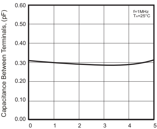
Fig.2 - Typical Capacitance Between Terminals Characteristics
