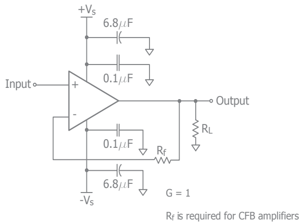
Figure 5. Typical Unity Gain (G=1) Circuit
