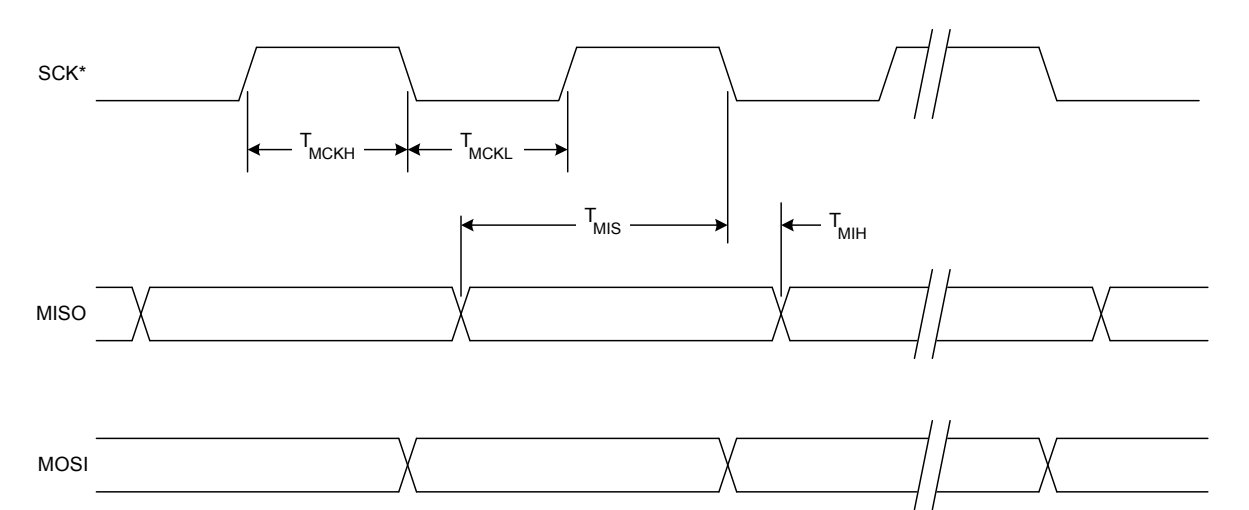
Figure 30.8. SPI Master Timing (CKPHA = 0)
