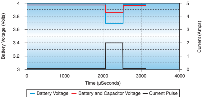
Figure 5. GSM Pulse
