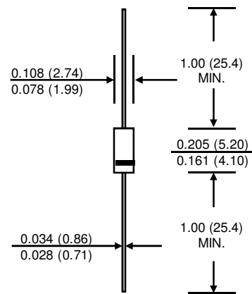
DO-41
