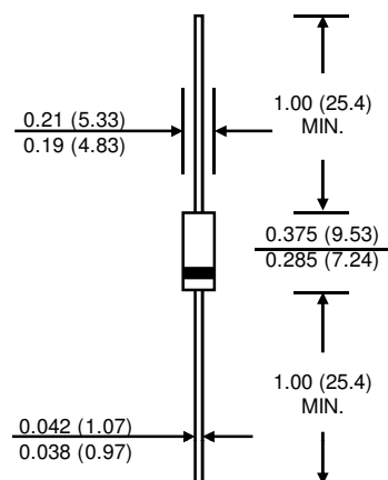
DO-201
