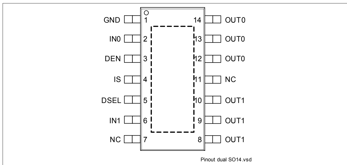
Figure 2 Pin Configuration
