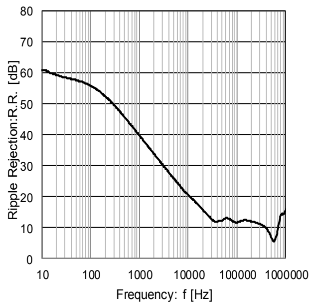
Figure 29. Ripple Rejection (Io=100mA)
