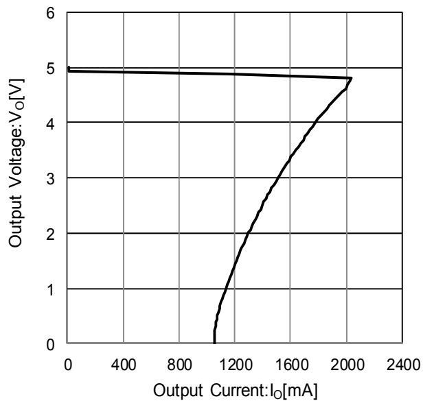
Figure 16. Load Regulation
