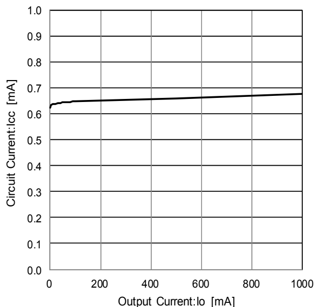
Figure 31. Circuit Current vs Output Current (Io = 0mA → 1000 mA)
