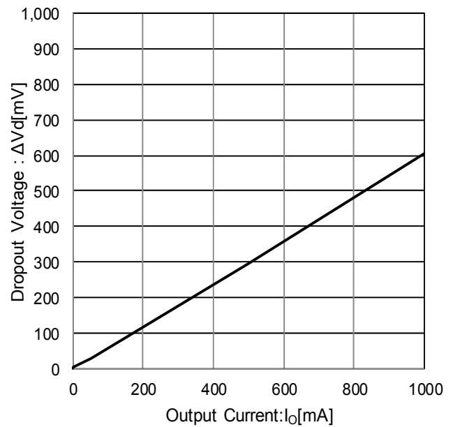
Figure 17. Dropout Voltage (V CC =4.75V) (I O =0mA→1000mA)
