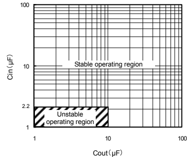
Cin vs Cout 1.0V \leq V_O < 3.0V Cout and Ceramic capacitor 10 \mu F is connected in parallel. (Reference data)
