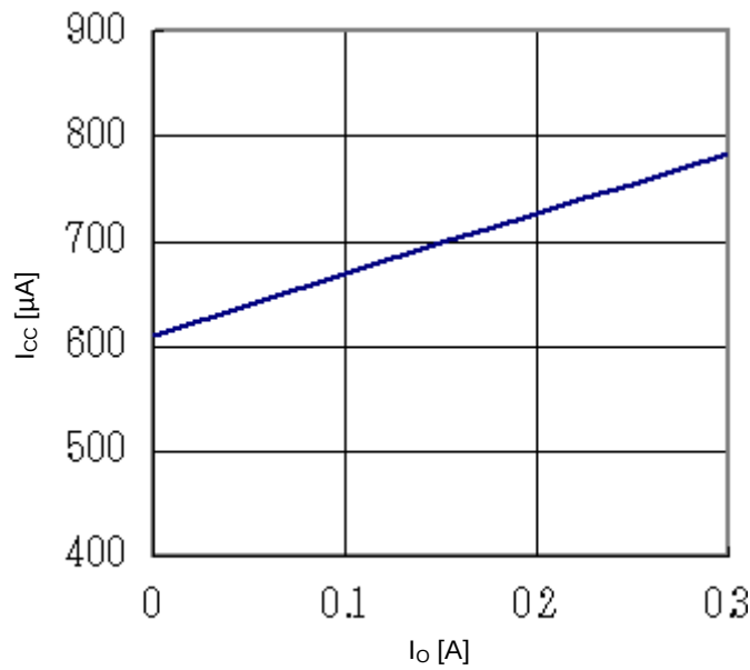
Figure 20. I_o - I_{cc}
