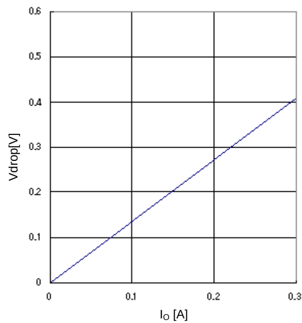
Figure 22. Minimum dropout Voltage 2 ( V_{CC}=4.5 V, T_a=25^\circ C )
