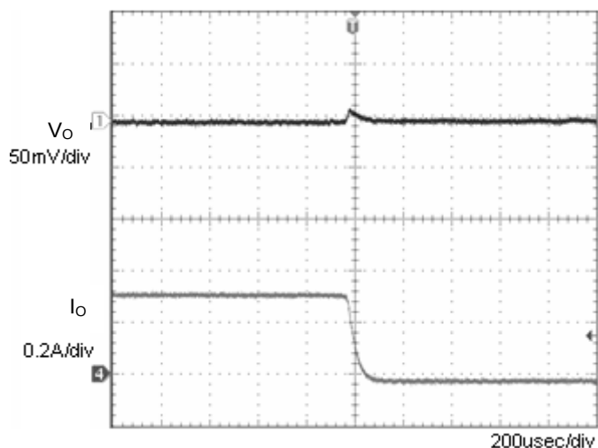
Figure 4. Transient Response (0.3→0A) C_o=1\mu\text{F}
