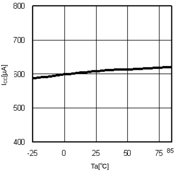
Figure 10. T_a-I_{cc}
