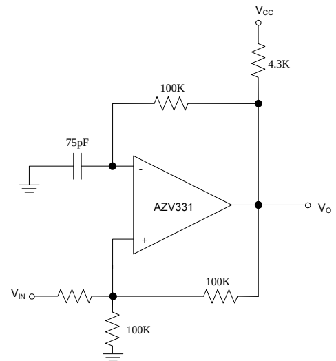
Squarewave Oscillator
