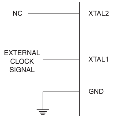
Figure 21. External Clock Drive Configuration
