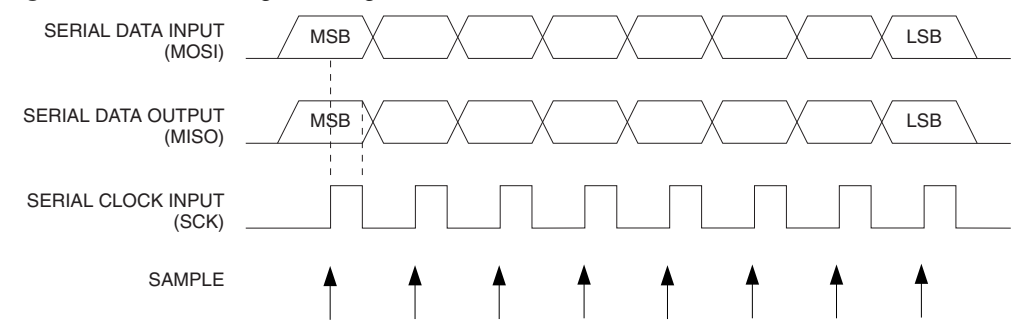
Figure 85. Serial Programming Waveforms
