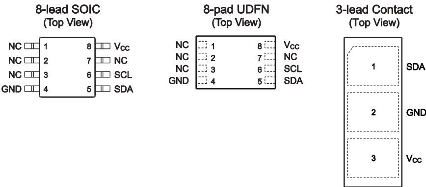
Figure 1. Pinouts
