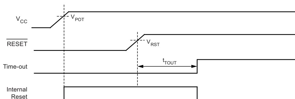
Figure 16-3. MCU Start-up, RESET Extended Externally
