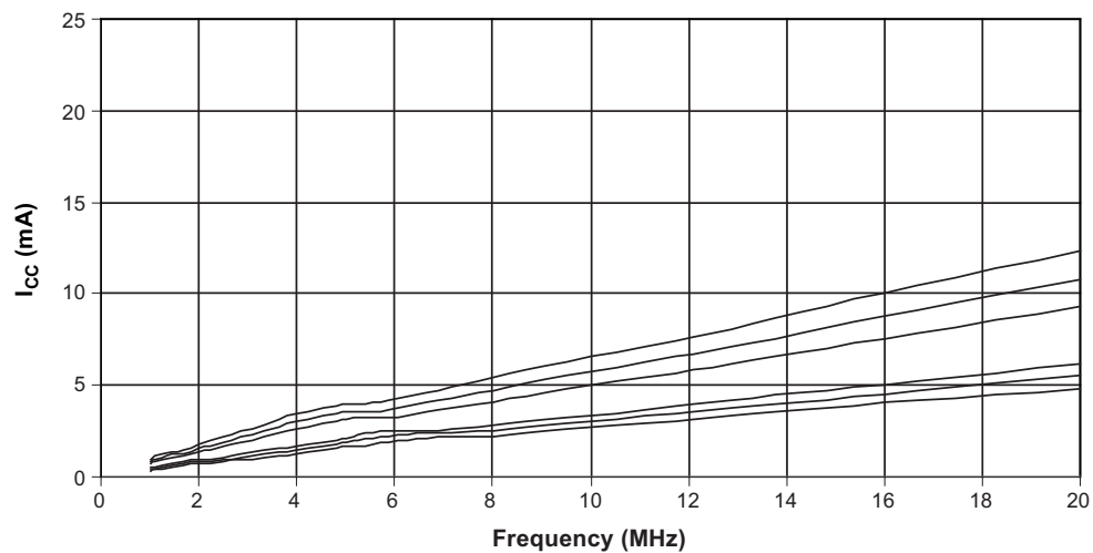
Figure 30-3. Active Supply Current versus frequency (1 to 20MHz) - Temp. = 25°C
