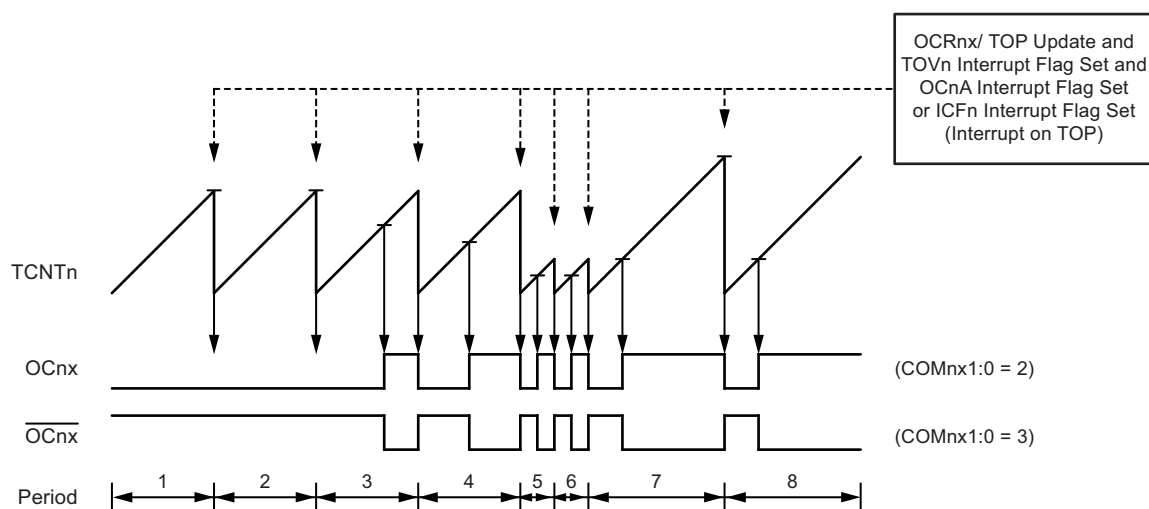
Figure 21-7. Fast PWM Mode, Timing Diagram
