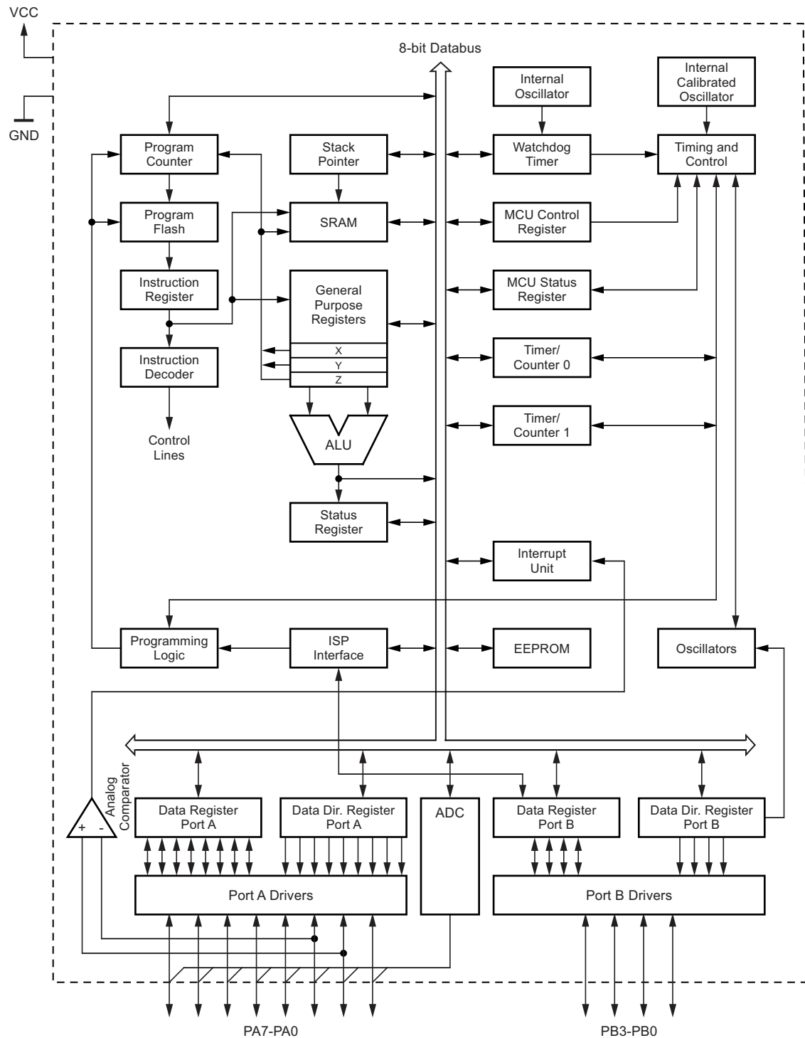
Figure 9-1. Block Diagram
