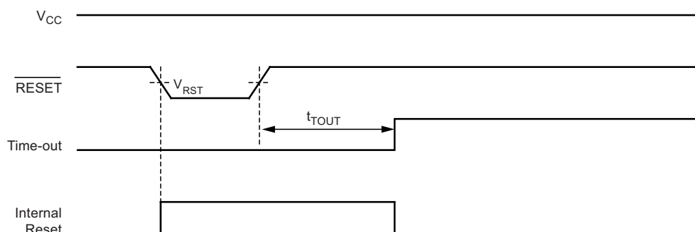
Figure 16-4. External Reset During Operation
