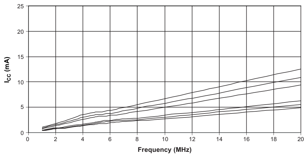
Figure 30-4. Active Supply Current versus frequency (1 to 20MHz) - Temp. = 125°C
