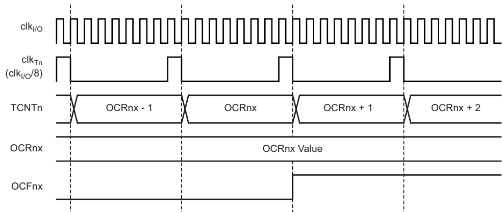
Figure 20-10. Timer/Counter Timing Diagram, Setting of OCF0x, with Prescaler ( f_{\text{clk\_I/O}}/8 )
