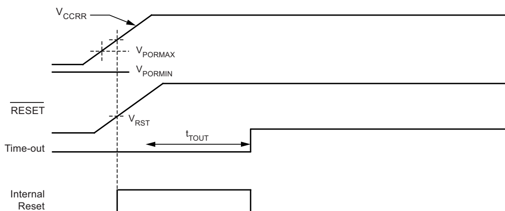
Figure 16-2. MCU Start-up, RESET Tied to V_{CC}
