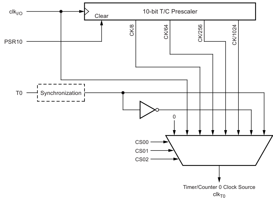
Figure 22-2. Prescaler for Timer/Counter0
