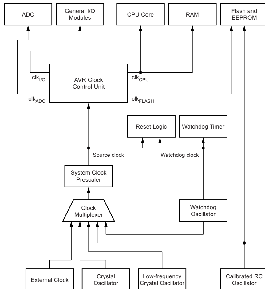
Figure 14-1. Clock Distribution
