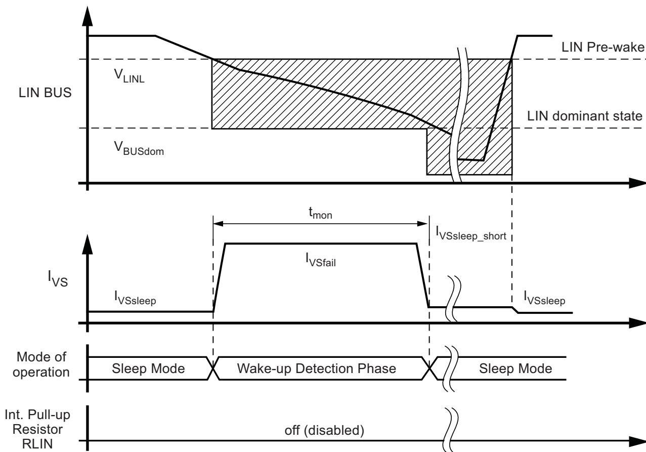
Figure 4-4. Floating LIN Bus During Sleep Mode
