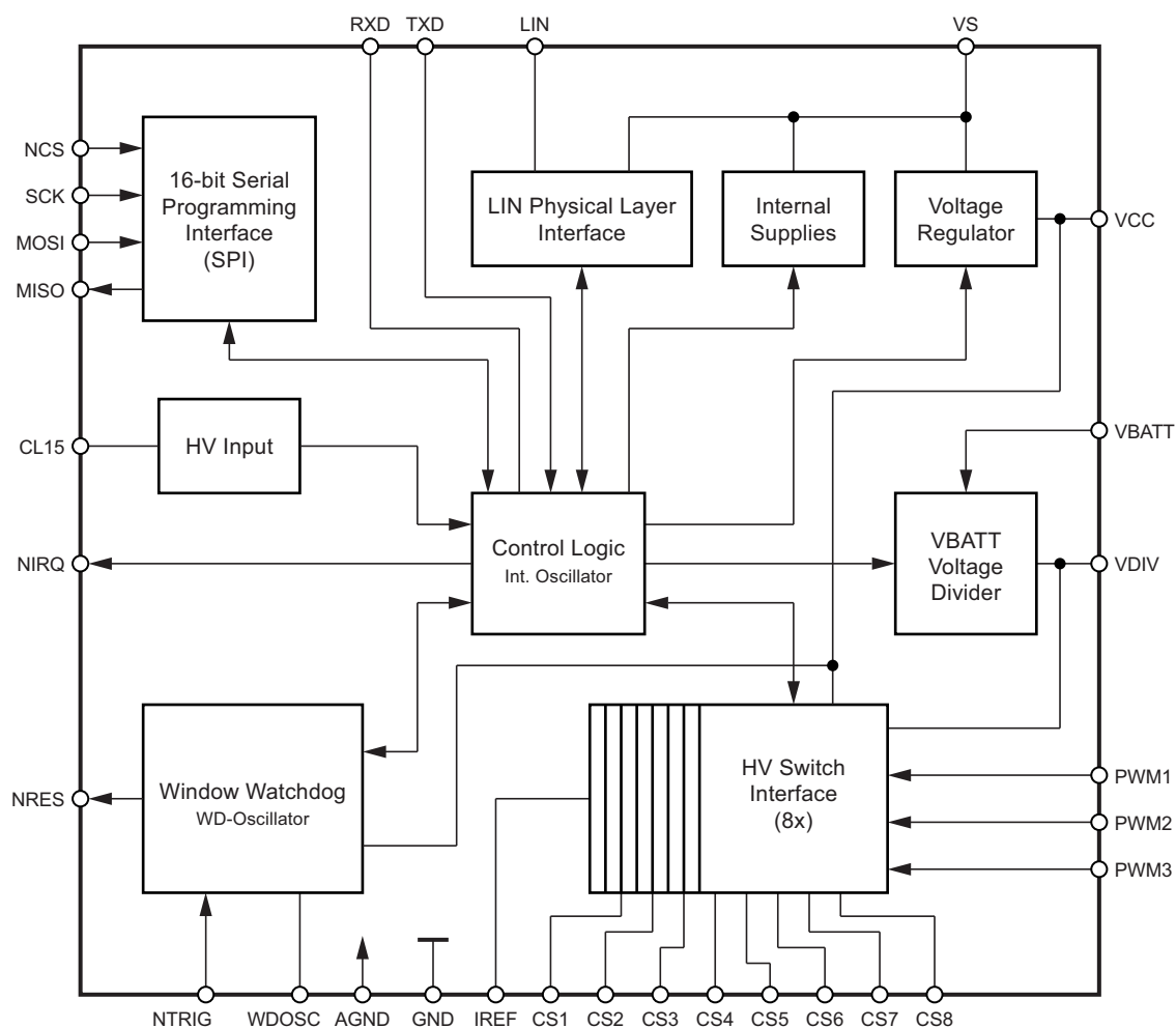
Figure 1-1. Block Diagram
