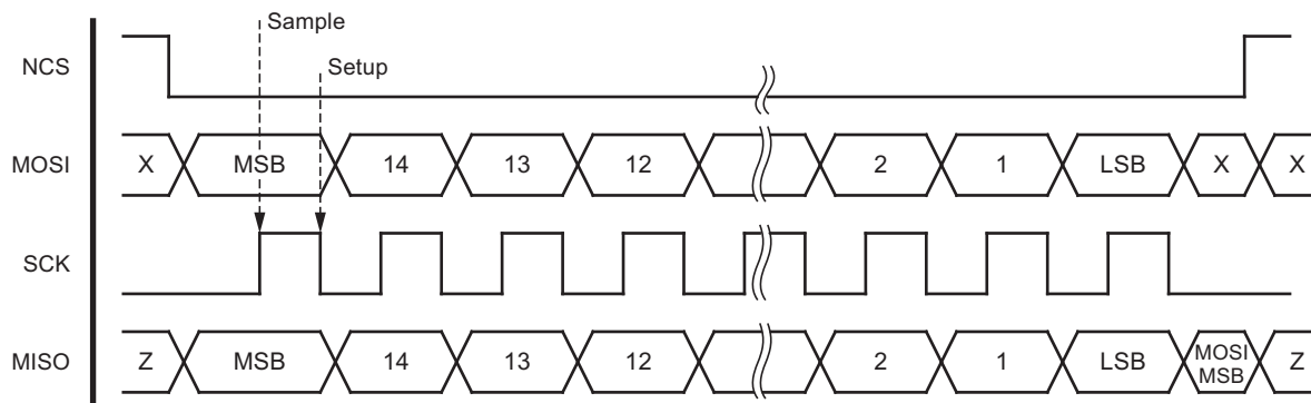
Figure 7-1. POL = 0 / PHA = 0 Setup
