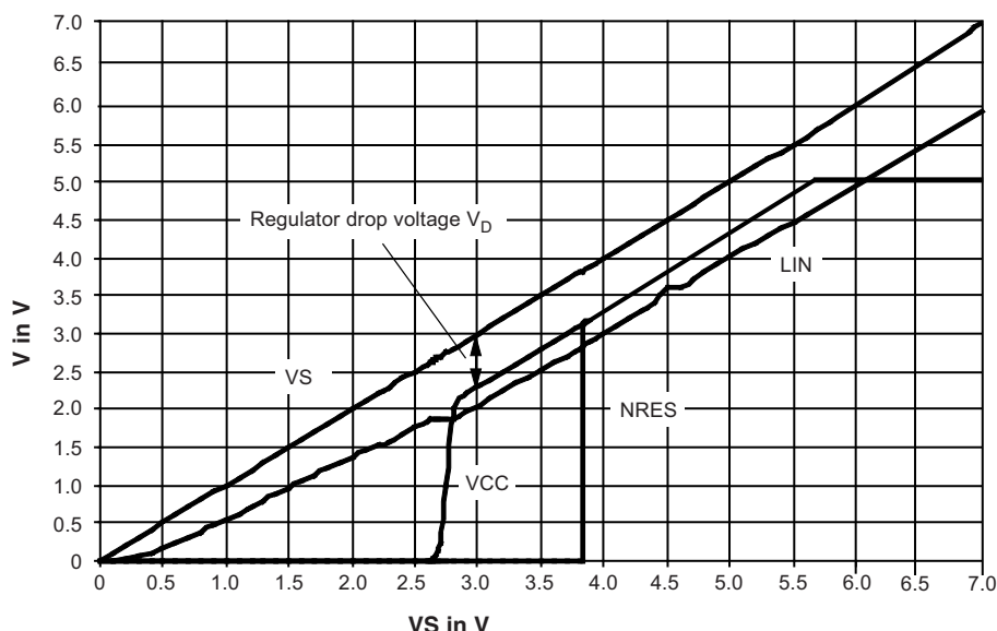
Figure 4-8. VCC versus VS
