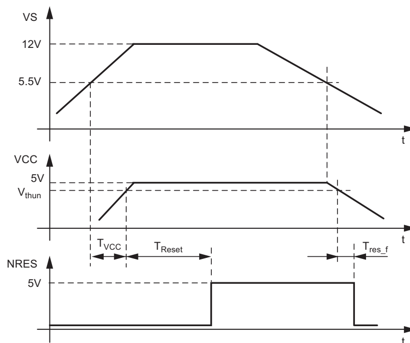
Figure 9-1. VCC Voltage Regulator: Ramp-up and Undervoltage Detection
