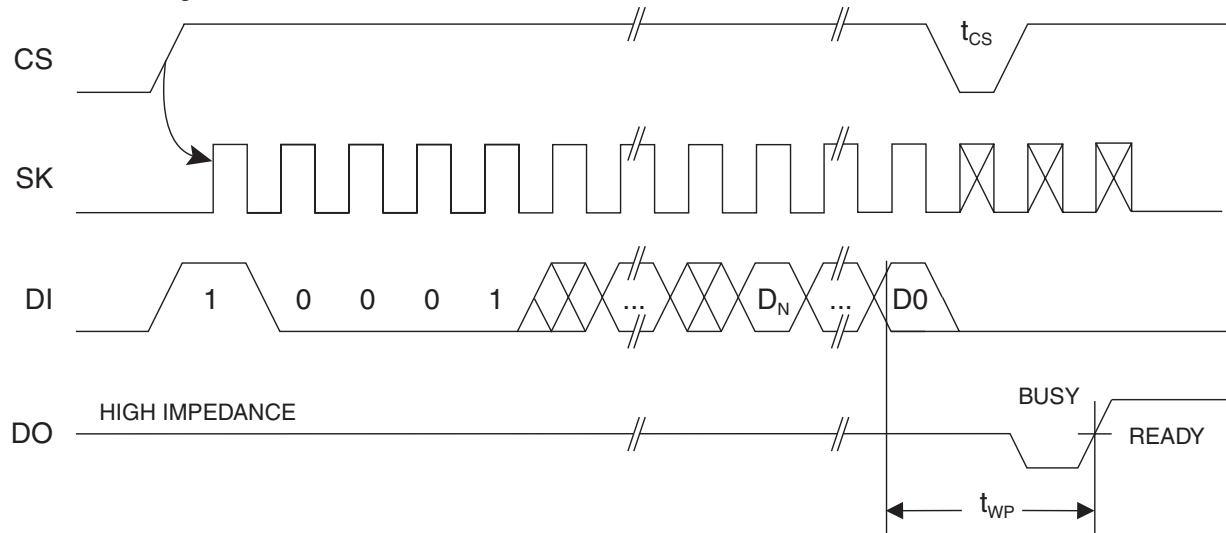
Figure 7. WRAL Timing (1)
