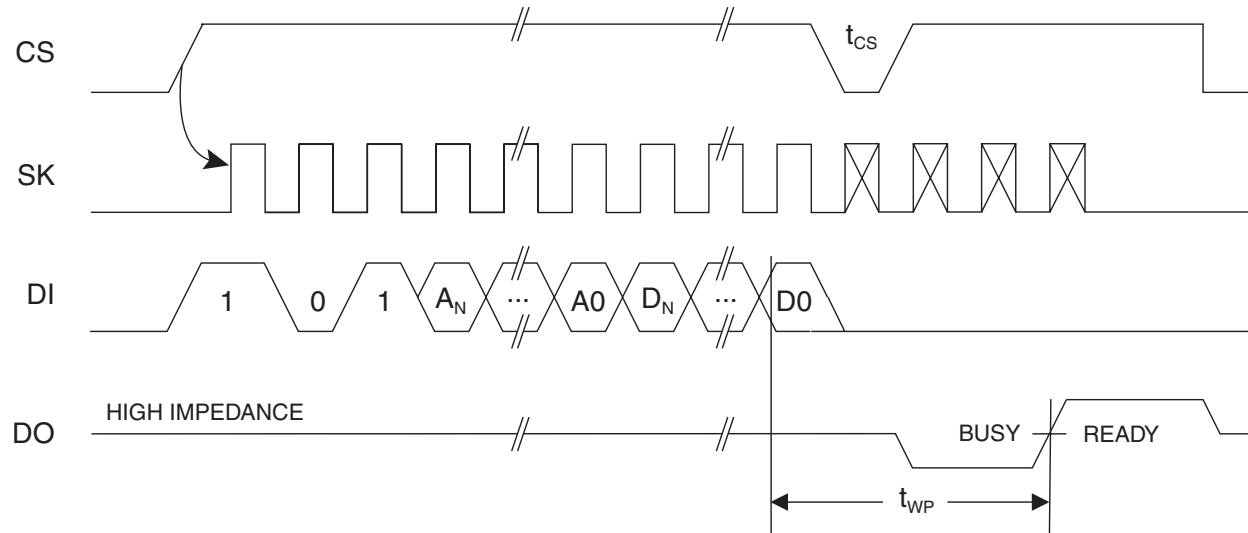
Figure 6. WRITE Timing
