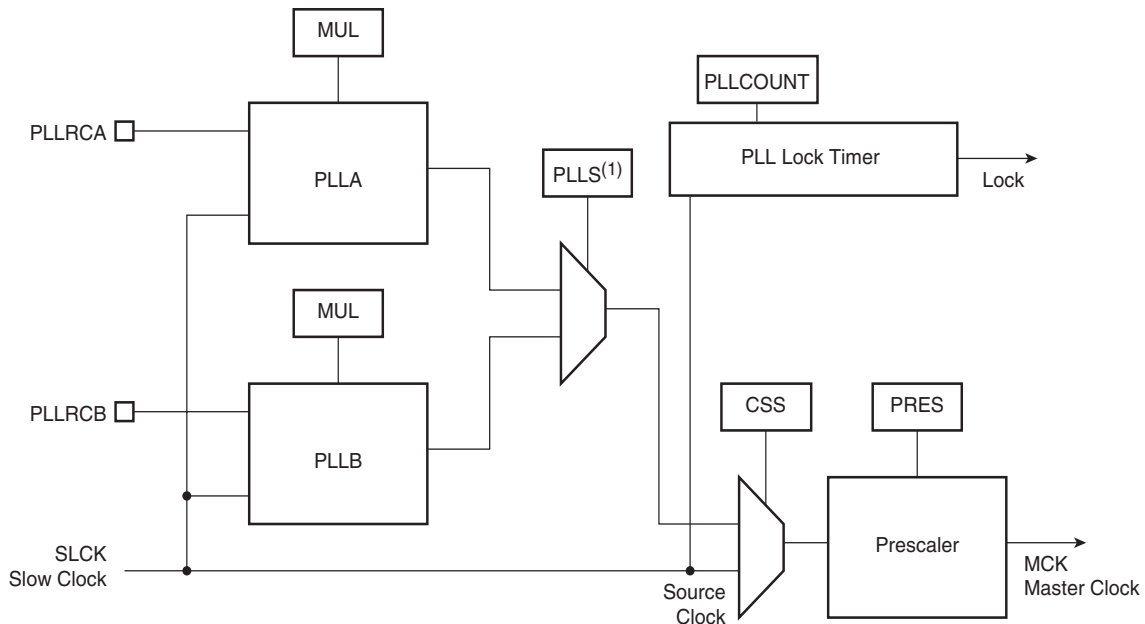
Figure 12-4. Master Clock
