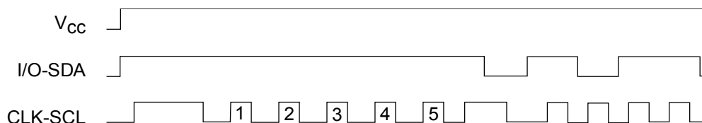
Figure 7-1. Start-up Sequence
