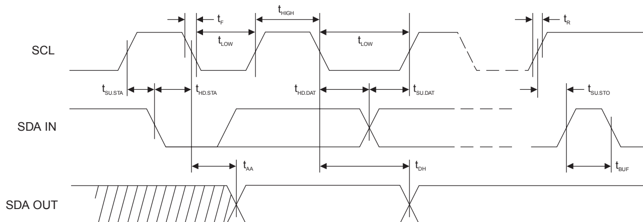
Figure 11-1. Bus Timing
