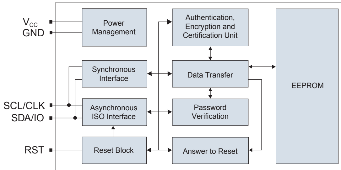
Figure 2-1. Block Diagram
