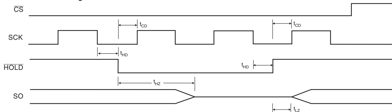
Figure 3-8. \overline{\text{HOLD}} Timing
