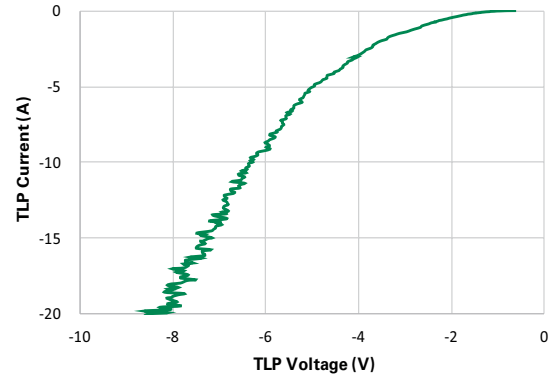
AQHV24 Negative Transmission Line Pulsing(TLP) Plot
