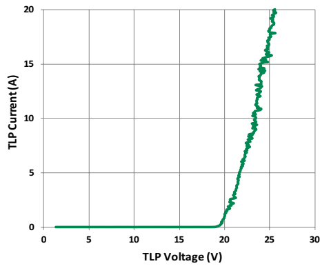
AQHV15 Positive Transmission Line Pulsing (TLP) Plot
