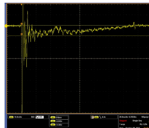
AQHV15 -8kV Contact ESD Clamping Voltage
