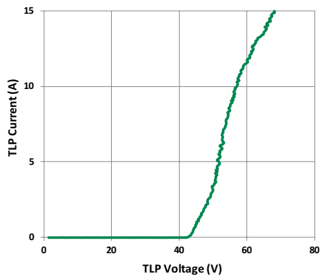
AQHV36 Positive Transmission Line Pulsing(TLP) Plot
