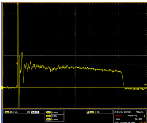
AQHV24 +8kV Contact ESD Clamping Voltage
