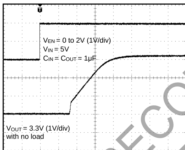
Start-Up Time
