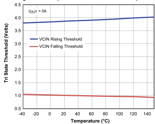
Fig 12. PWM Input Tristate Threshold vs. Temperature
