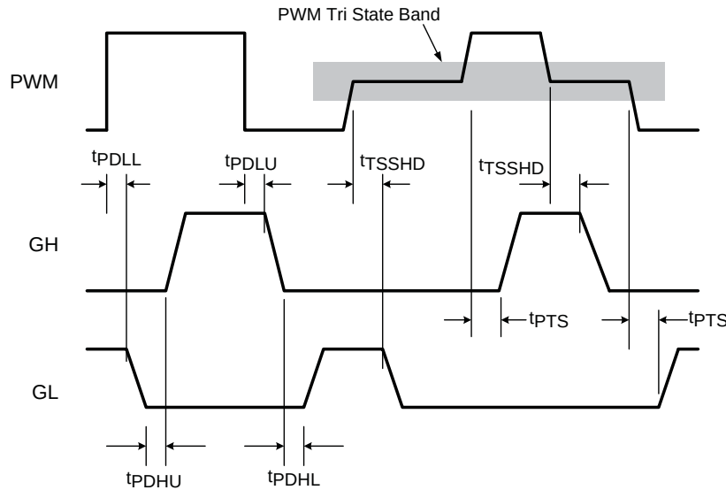
Figure 16. Timing Diagram
