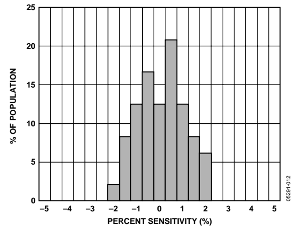
Figure 12. Z vs. X Cross-Axis Sensitivity
