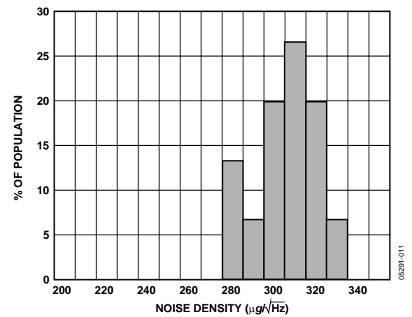
Figure 11. X-Axis Noise Density at 25°C
