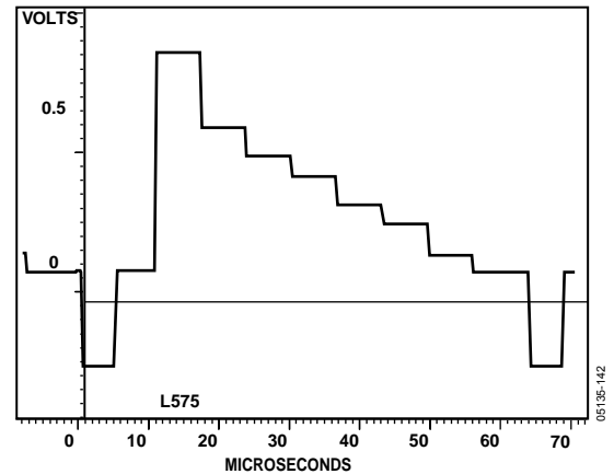
Figure 140. PAL Chroma
