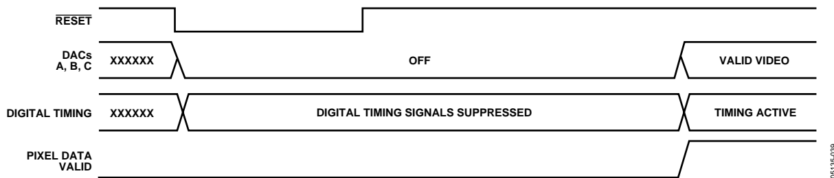
Figure 62. \overline{\text{RESET}} Timing Sequence
