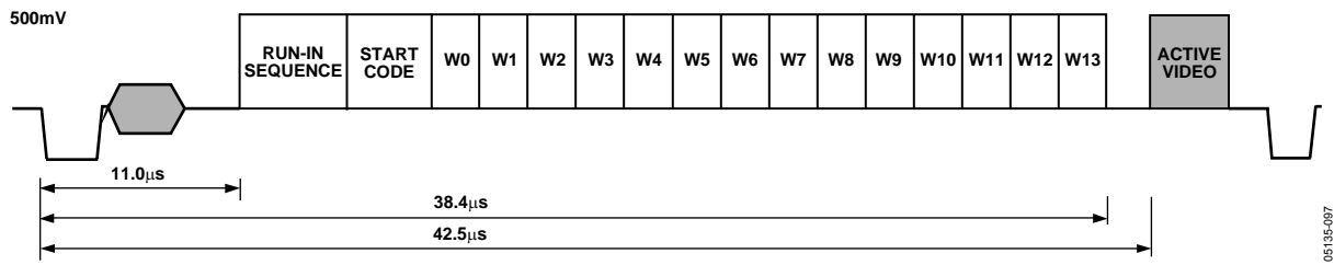
Figure 96. WSS Waveform Diagram
