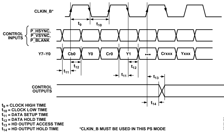
Figure 6. PS 4:2:2 8-Bit Interleaved at 27 MHz \overline{\text{HSYNC}} / \overline{\text{VSYNC}} Input Mode (Input Mode 100)
