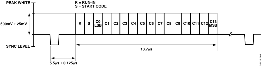
Figure 92. PS 625p CGMS-A Waveform (Line 43)
