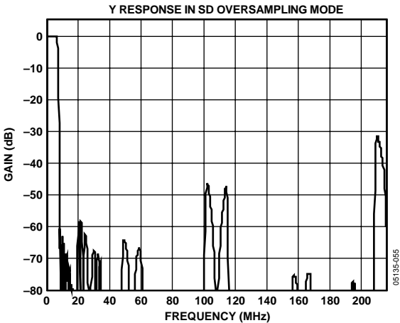
Figure 30. SD—Y: 16x Oversampling Filter
