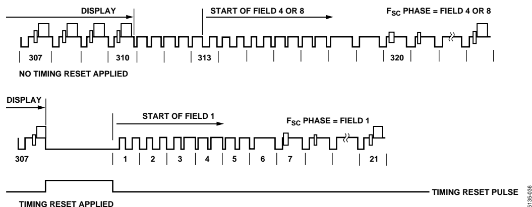
Figure 59. Timing Reset Diagram
