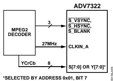
Figure 48. SD Only Input Mode
