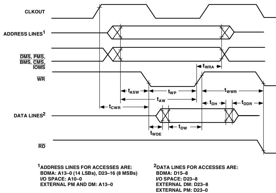
Figure 30. Memory Write
