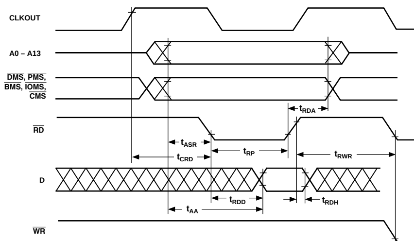
Figure 18. Memory Read
