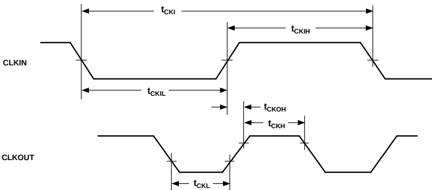
Figure 15. Clock Signals
