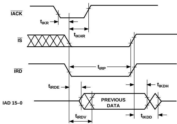
Figure 25. IDMA Read, Short Read Cycle
