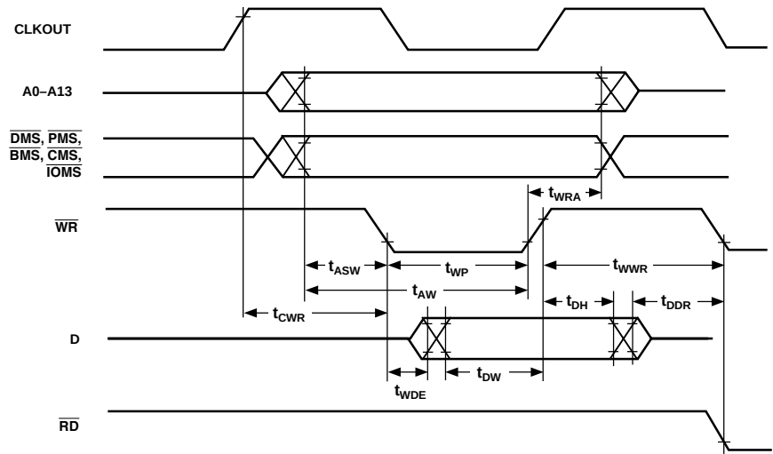
Figure 19. Memory Write
