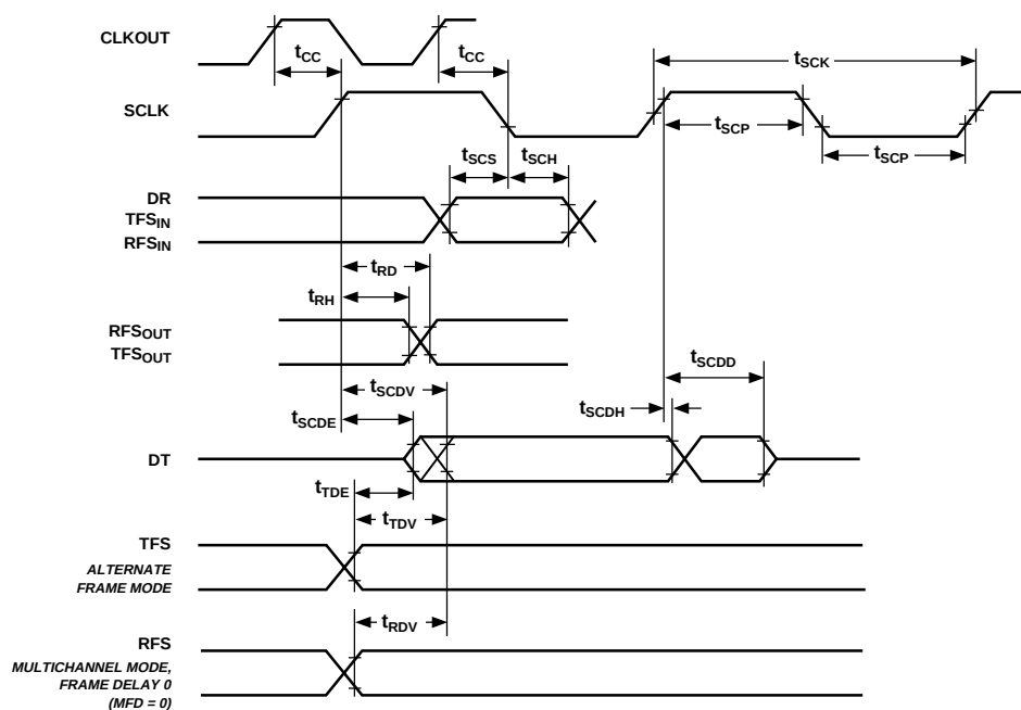
Figure 20. Serial Ports
