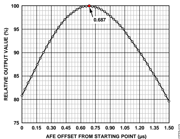
Figure 18. AFE Sweep Example
