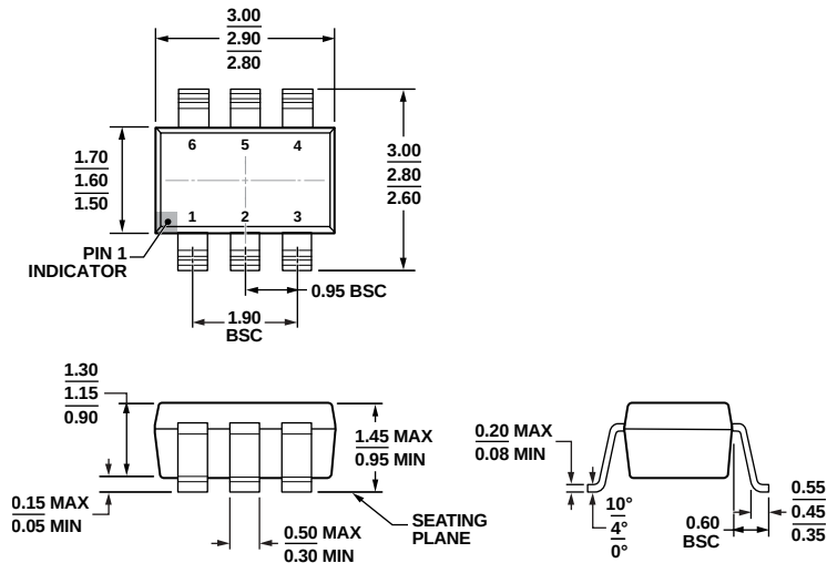
COMPLIANT TO JEDEC STANDARDS MO-178-AB Figure 7. 6-Lead Small Outline Transistor Package [SOT-23] (RJ-6) Dimensions shown in millimeters
