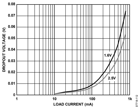
Figure 12. Dropout Voltage vs. Load Current, V_{OUT} = 1.6\text{ V}, 2.5\text{ V}
