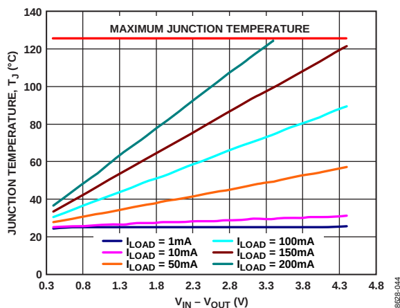
Figure 46. 100 mm 2 of PCB Copper, TSOT, T_A = 25^{\circ}\text{C}
