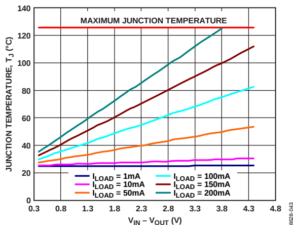
Figure 45. 500 mm 2 of PCB Copper, TSOT, T_A = 25^{\circ}\text{C}
