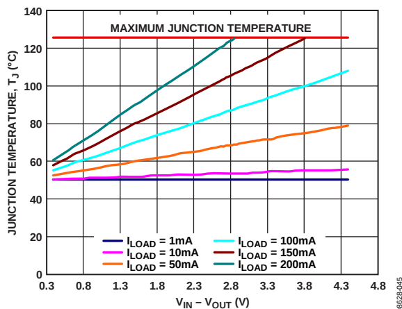
Figure 47. 500 mm 2 of PCB Copper, TSOT, T_A = 50^{\circ}\text{C}
