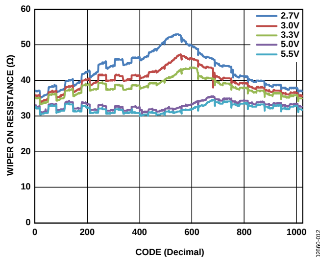
Figure 9. Wiper On Resistance vs. Code
