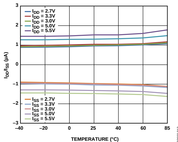
Figure 10. I_{DD} vs. Temperature, R_{AB} = 25\text{ k}\Omega
