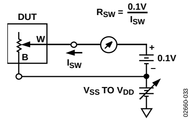
Figure 23. Incremental On Resistance
