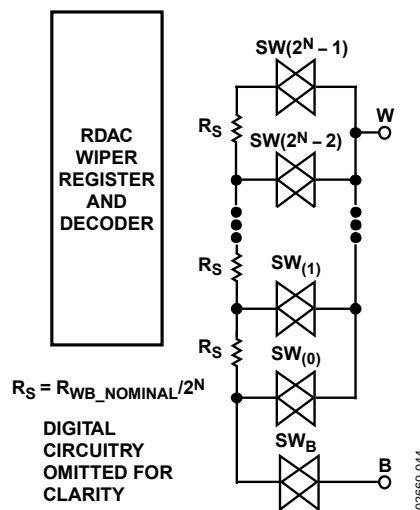
Figure 32. Equivalent RDAC Structure
