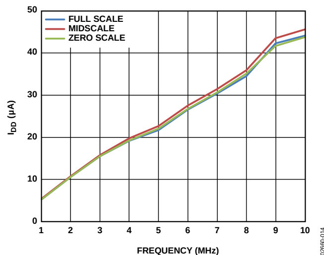
Figure 11. I_{DD} vs. Clock Frequency
