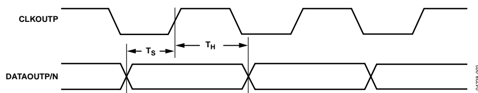
Figure 2. Output Timing
